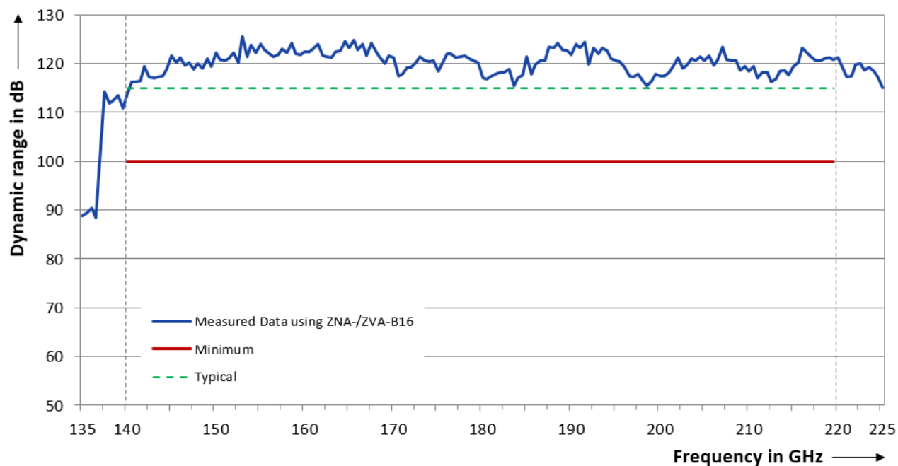
Dynamic range versus frequency of the R&S®ZC220
