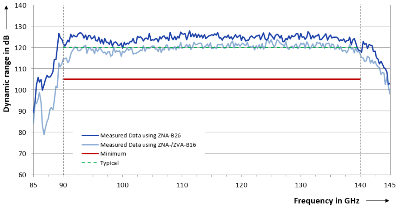
Dynamic range versus frequency of the R&S®ZC140
